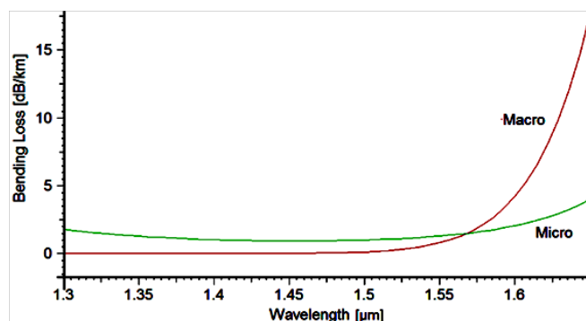
Figure 3 Bending losses of the designed NZDSF profile versus wavelength.
