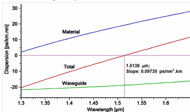
Figure 2 Dispersion of the designed NZDSF profile versus wavelength. 1.5138 \mu\text{m} , Slope: 0.09730 \text{ps}/\text{nm}^2\cdot\text{km}
