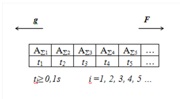
Figure 1 The diagram of the summary potential A_{\Sigma} change in the process when matter flies away from the SN explosion for the non-gauge force action realization.
