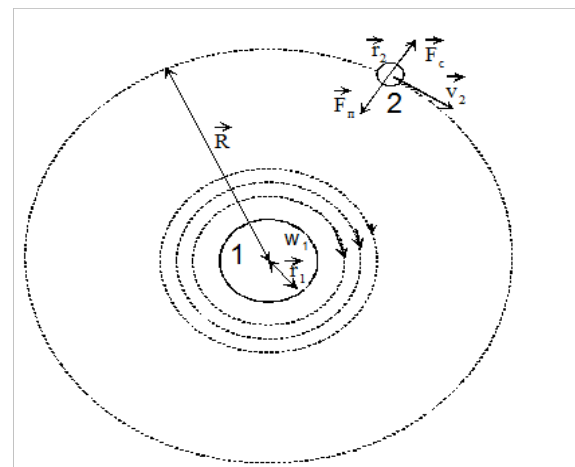
Figure 1 Two-dimensional model of the gravitational interaction between the two bodies.
