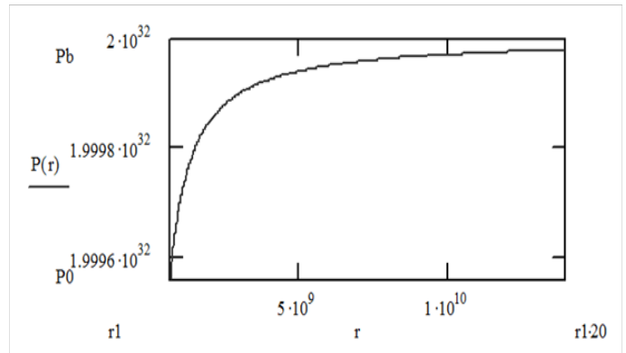
Figure 2 Radial distribution of ether pressure for the Sun.
