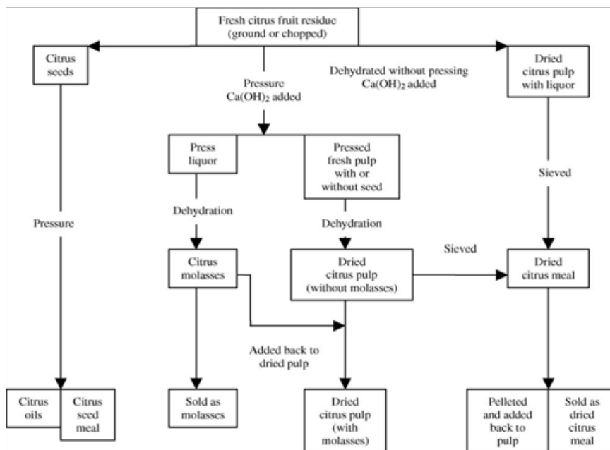
Figure 1 Schematic presentation of citrus by-product production Sinclair. 43
