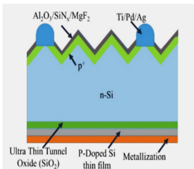
Figure 6 TOPCon solar cell visual diagram. Reprinted from [18].
