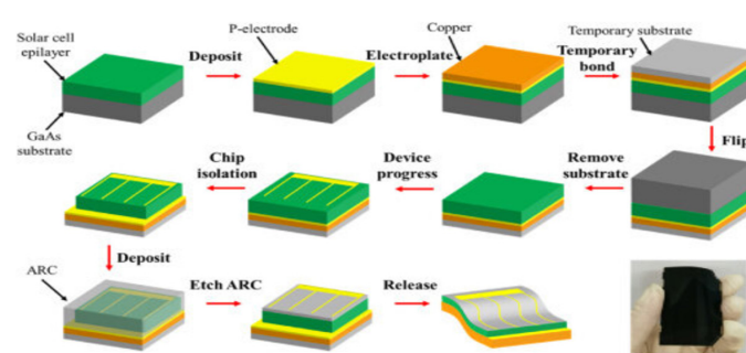
Figure 16 A Visual Representation of the Fabrication Process for a Triple Junction Solar Cell. Reprinted from Luo X, et al. 45
