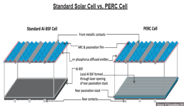
Figure 4 A schematic comparison of standard BSF solar cells VS. a PERC cell. Reprinted from Chunduri, et al. 12
