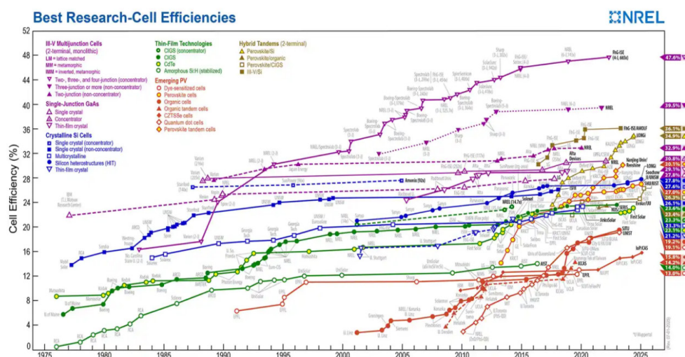
Figure 9 Best research-cell efficiency chart. Reprinted from NLR. 22
