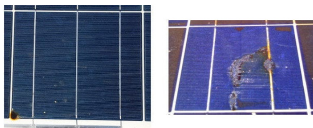
Figure 22 An Image of a Hot Spot Fault. Reprinted from Andrews R, et al. 82
