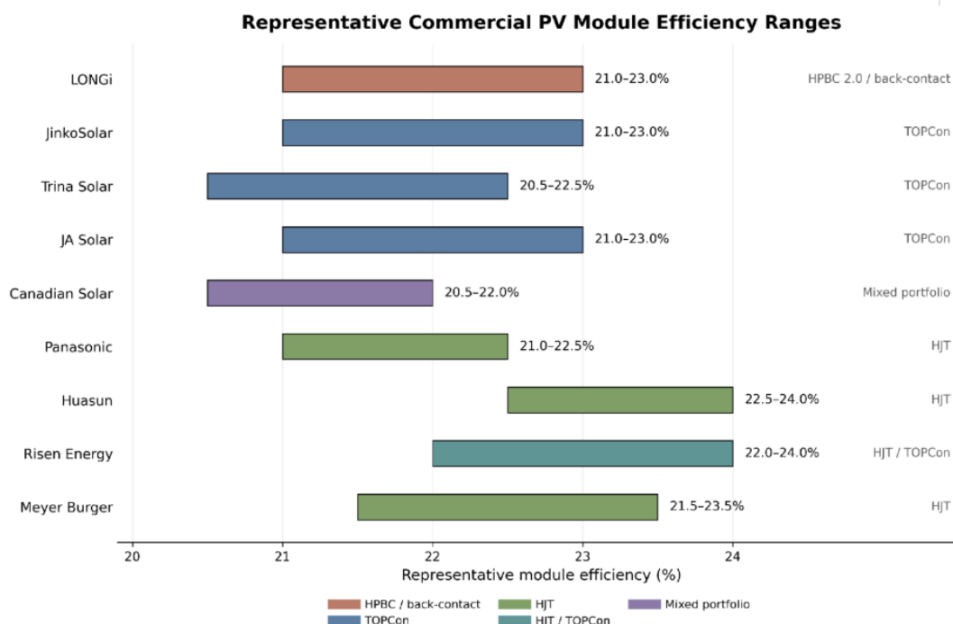
Figure 10 Representative commercial PV module efficiency ranges.
