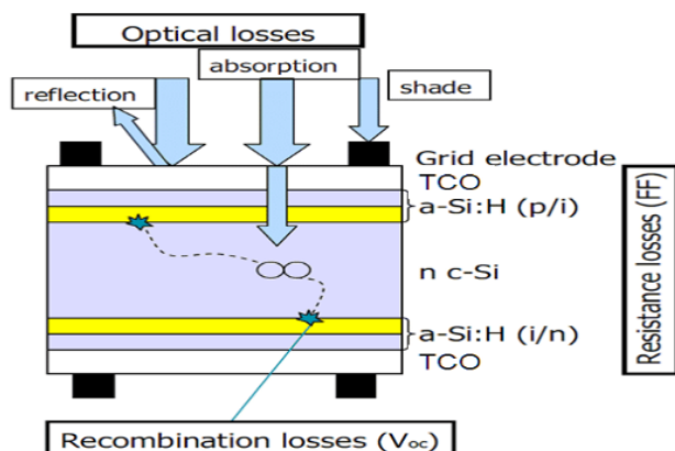
Figure 2 A visual representation of the various loss mechanisms in solar cells. Reprinted from Ling. 13
