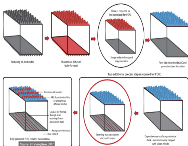
Figure 5 A flowchart of the processing sequence of a PERC cell. Reprinted from Chunduri, et al. 12
