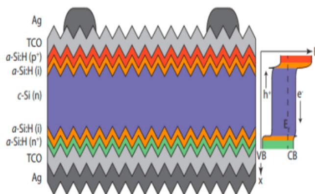
Figure 8 Schematic of a bifacial HJT Solar Cell. Reprinted from DeWolf, et al. 21
