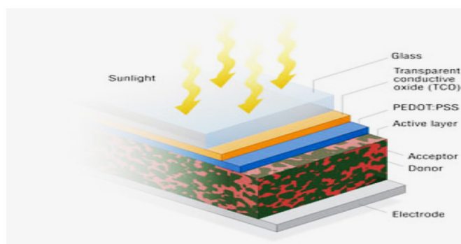
Figure 13 A Visual Diagram for an OPV. Reprinted from US Department of Energy. 40
