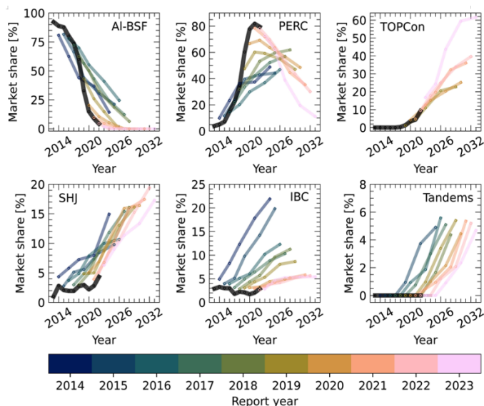
Figure 3 Silicon Solar Cell Architecture Market Projections. Reprinted from Stefani et al. 15
