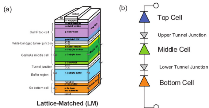
Figure 15 A Visual Representation of a Triple Junction Solar Cell. Reprinted from Cotal H, et al. 44
