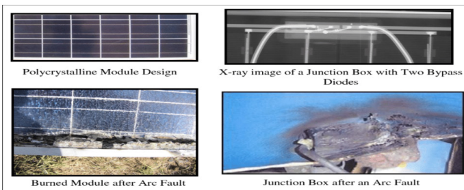
Figure 23 Several Images of an Arc Fault. Reprinted from Johnson J, et al. 83
