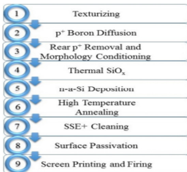
Figure 7 TOPCon solar cell fabrication process flowchart. Reprinted from
