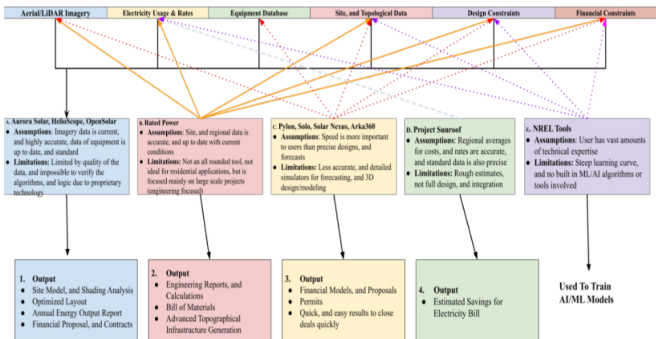
Figure 27 A block diagram of software tools for pre-design and optimization.
