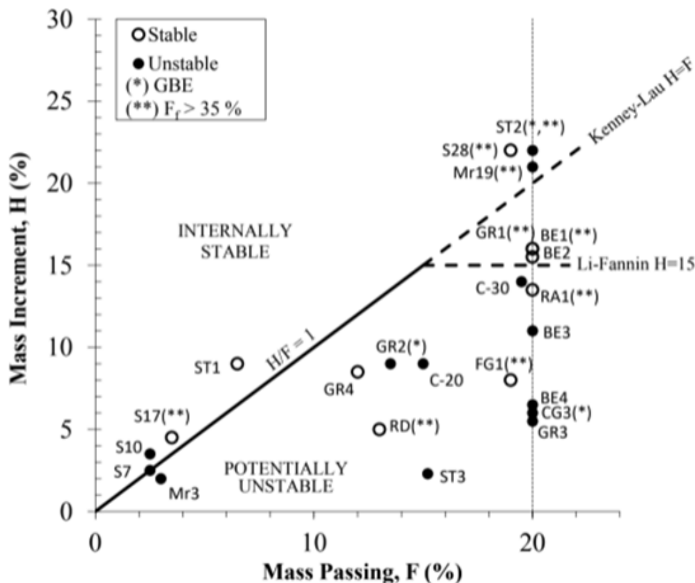
Figure 2 Summary of gradation analyses: the Kenney & Lau 15,16 method and the Li & Fannin 17 adaptation.
