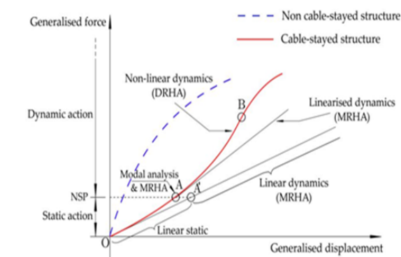
Figure 1: Qualitative difference between the load-displacement response of classical cable-stayed bridges and structures without cable-system.
