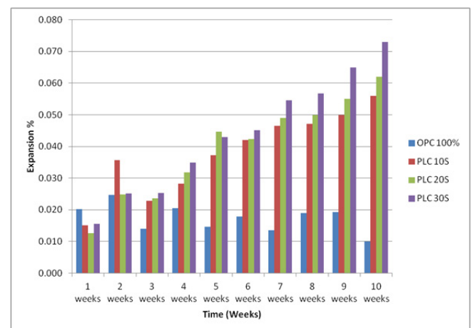
Figure 4 Average expansion length of 10 weeks of portland limestone mixtures.
