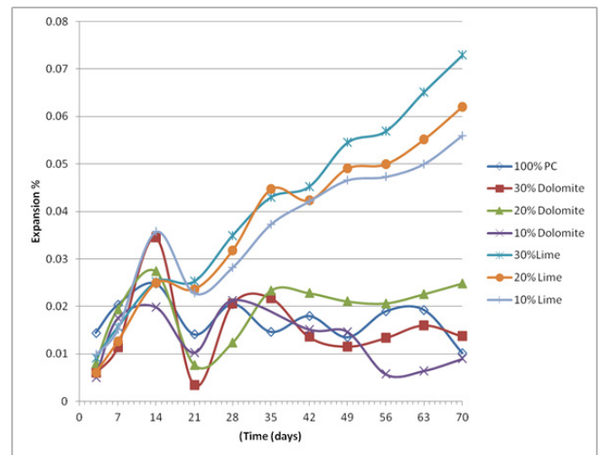
Figure 3 Average expansion due to sulfate attack during 70 days at 20°C.
