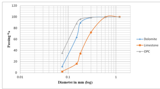
Figure 1 Particle size distribution for OPC, limestone and dolomite.
