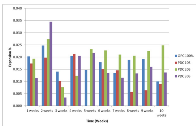
Figure 5 Average expansion length of 10 weeks of portland dolomite mixtures.
