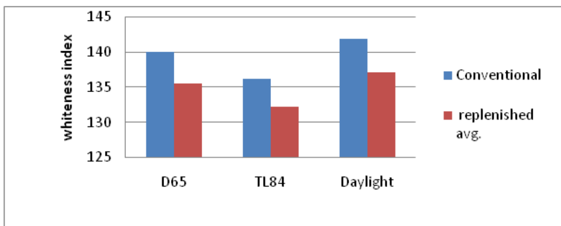
Figure 1 Whiteness index of Conventional & Replenished pretreated fabrics.
