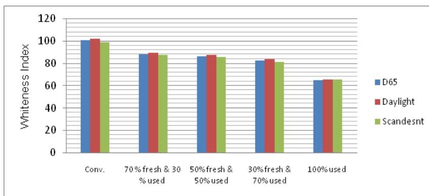
Figure 4 Whiteness index from bulk trial.
