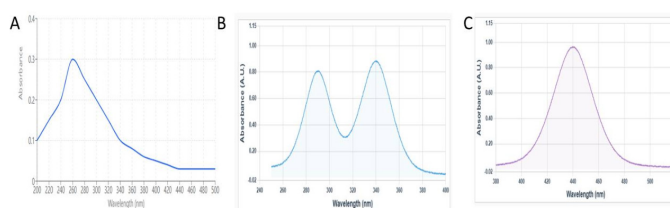
Figure 2 Ultraviolet visible Spectrum of (A) sodium selenite solution (B) Tetrapleura tetraptera Husk aqueous extract (C) selenium nanoparticles synthesized from Tetrapleura tetraptera husk aqueous extract.
