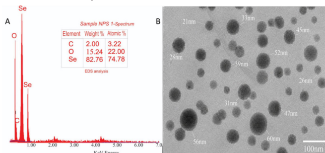
Figure 4 (A) The Energy Dispersive X-ray (EDX) micrograph (B) Transmission Electron Microscopy (TEM) micrograph of the synthesized selenium nanoparticles.
