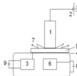
Figure 1 The experimental setup. 1 - metal cylinder; 2 Antenna “Sputnik”; 3 - high-voltage pulse generator; 4 - transparent conductive coating; 5 - transparent quartz electrode; 6 - video converter; 7 - glow; 8 - USB-drive; 9 - Power Supply.
