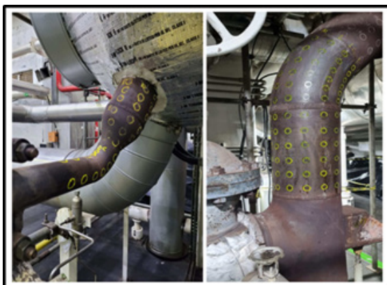
Figure 3 Angra 1 Systems Engineering determines the creation and formation of the GRID/MESH taking into account the diameter of the pipe, type of straight section (vertical/Horizontal) and type of curvilinear section (30, 45, 60, 90 or another value in degrees).
