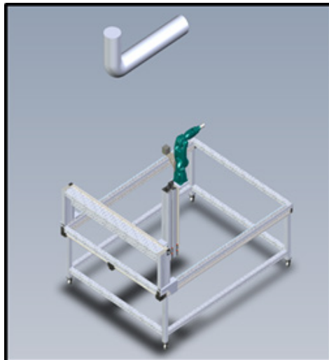
Figure 2 Complete SMRE system, containing the thickness measuring unit (URMC) and the remote unit (UROV).
