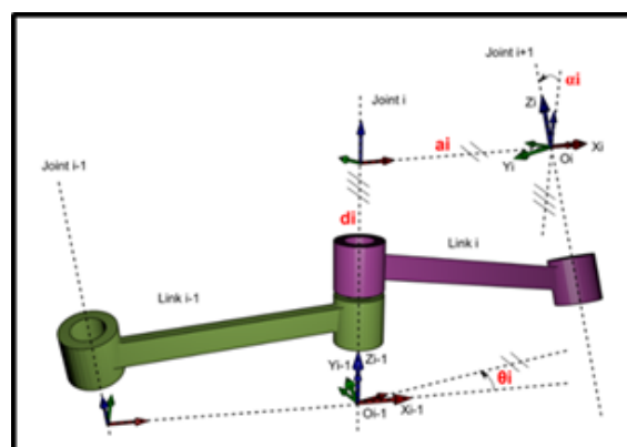
Figure 1 Classical Denavit-Hartenberg Notation. 5
