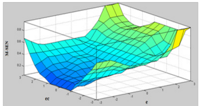
Figure 11 Surface plot corresponding to M-SEN.
