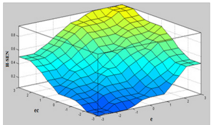
Figure 12 Surface plot corresponding to H-SEN.
