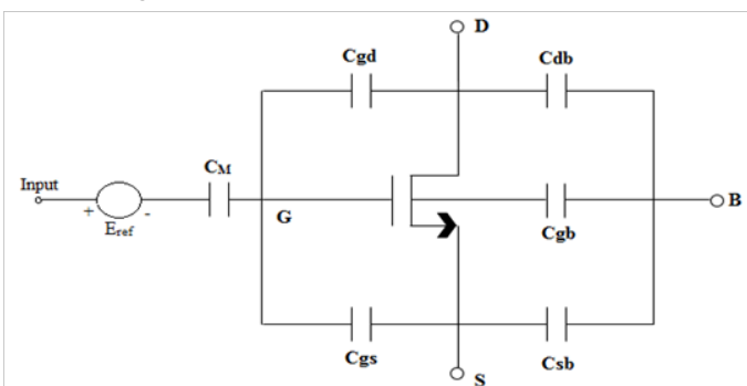
Figure 3 Circuit for PCS.
