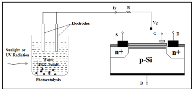
Figure 1 Photo catalysis process.
