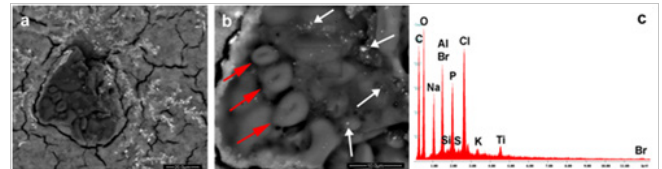
Figure 7 Image of an area in a Repevax drop where the morphology of red cells (red arrows) were identified. It is impossible to know whether they are human or animal origin. Among the debris of saline and Aluminum phosphate, there is the presence of debris (white arrows) composed of Aluminum, Bromine, Silicon, Potassium, Titanium.
