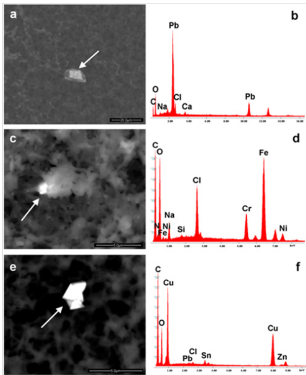
Figure 5 show particles surrounded by an organic compound. They are composed of Lead (a,b), Iron, Chromium, Nickel (stainless steel; c,d), Copper, Tin, Lead (e,f). The arrows show the points where EDS spectra were taken.
