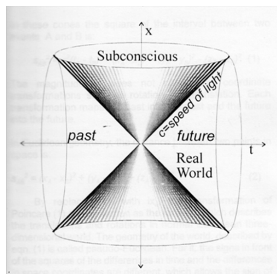
Figure 1 Minkovski's Four- Dimensional Representation of Einsteins Relativistic Theory.
