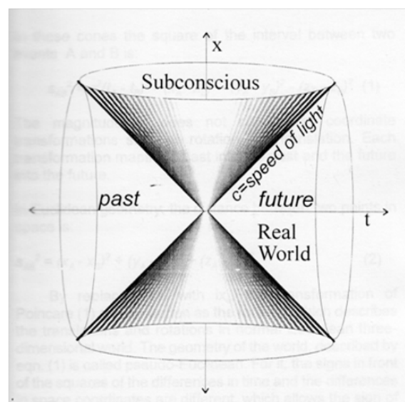
Figure 1 Minkovski's Four- Dimensional Representation of Einstiens Relativistic Theory.
