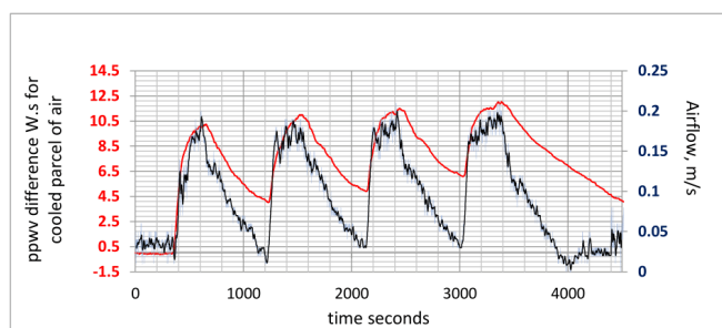
Experiment June 27th, 2016. The graph shows 4 refrigeration cycles. The left-hand axis shows the partial pressure change in water vapour in watt.seconds during the refrigeration cycle and the right-hand axis shows the anemometer readings in metres per second. The airflow was measured using a 2D- anemometer ©Peter Bunyard
