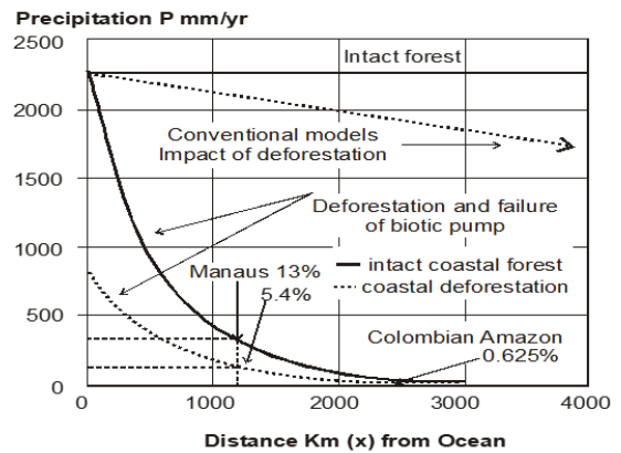
Widespread deforestation in the Amazon Basin would lead, according to the biotic pump theory of A. Makarieva and V. Gorshkov, to an exponential reduction in rainfall as one passed from the coast to the deep interior. The net result would be desert conditions and not the savannah-like conditions indicated by conventional (without biotic pump) climate models. ©Peter Bunyard
