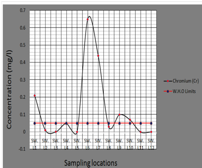
Figure 7 Chromium (Cr) concentration plot in surface water.
