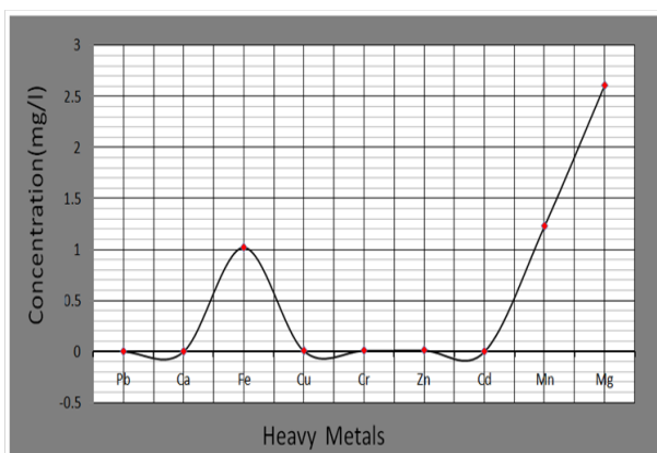
Figure 5 Heavy metals concentrations.
