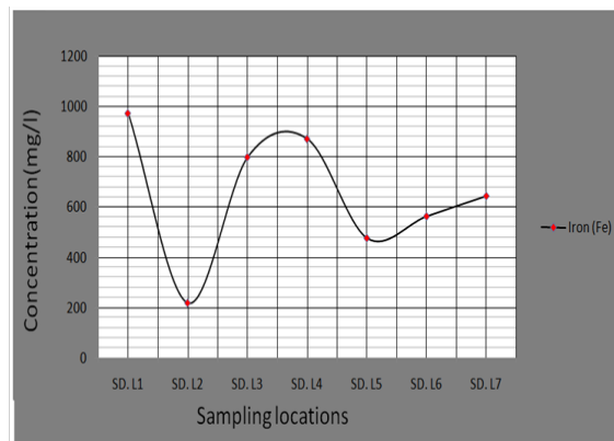
Figure 6 Plot of Iron (Fe) concentration in river sediments.
