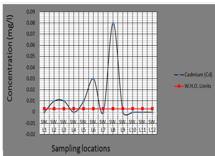
Figure 9 Plot of Cadmium (Cd) concentration in surface water.
