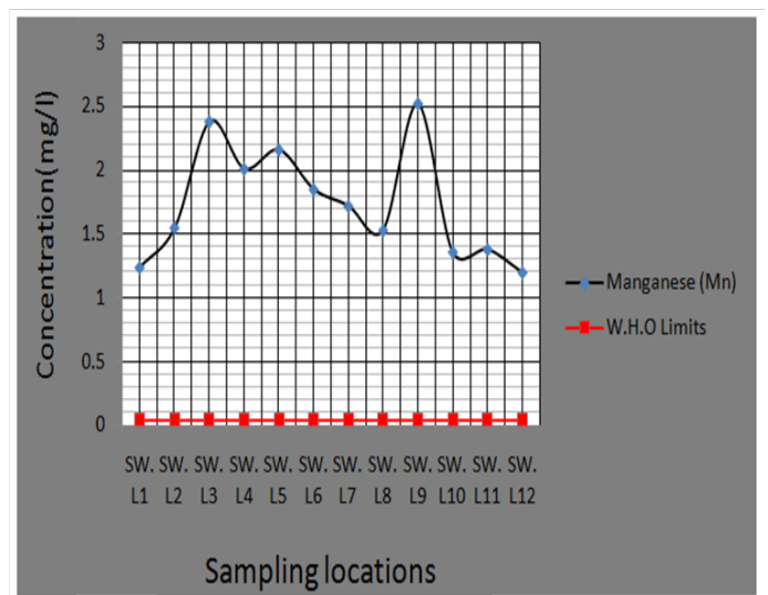
Figure 10 Manganese (Mn) concentration plot in surface water.
