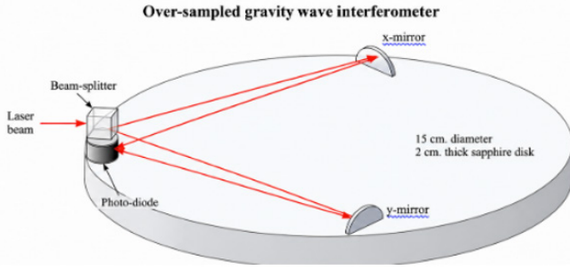
Figure 5 Schematic arrangement of interferometer components. Coherent beams reflect off the x — and y — mirrors; when they strike the photodiode they exit the interferometer. Output is sampled in discrete intervals: the intensity pattern is reconstructed using sampling algorithms. Each sample is independent, there is no multiple reflection.
