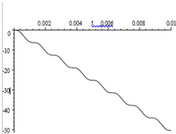
Figure 3 Mirror response in units of gravitational wave amplitude h to incoming gravity wave of maximum frequency \omega = 2\pi \times 800\text{s}^{-1} and duration 10ms. Suspension frequency is set at 1Hz.
