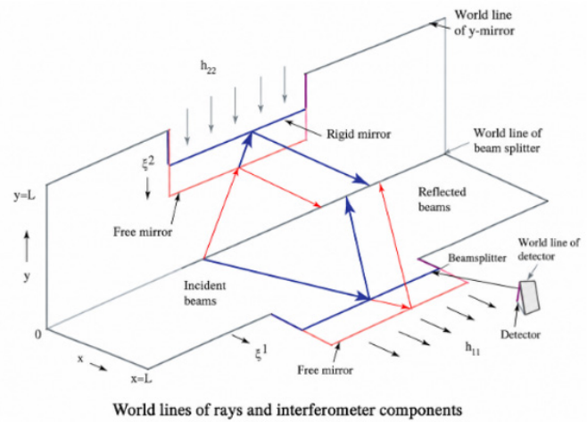
Figure 2 World lines of rays and interferometer components. Two mirror mounts, free in light and rigid in heavy lines, are shown under the influence of a gravity wave of constant amplitude h_{\mu\nu} . Although the surfaces are shown as planes they are saddle-shaped as in figure 1. The reflection points depend on the type of mirror mount, and so does the excess phase.
