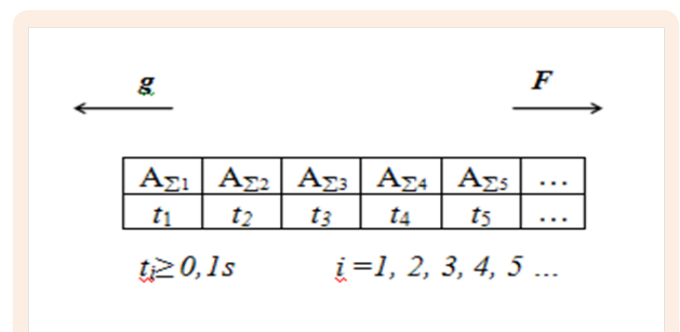
Figure 1: The diagram of the summary potential A_\Sigma change in the process when matter flies away from the SN explosion for the non-gauge force action realization.
