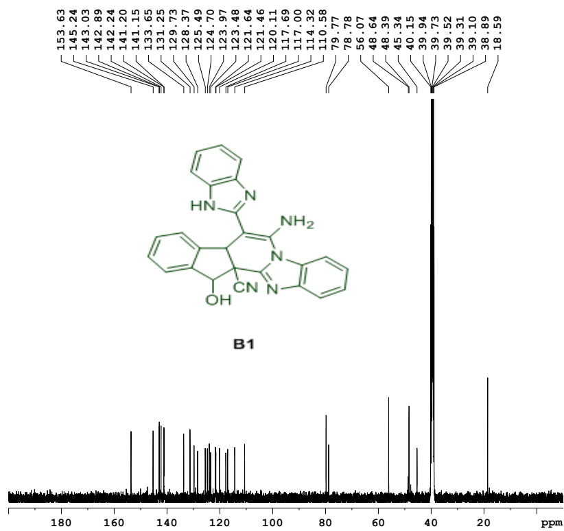
Figure 2 13 C NMR spectra of compound B1.
