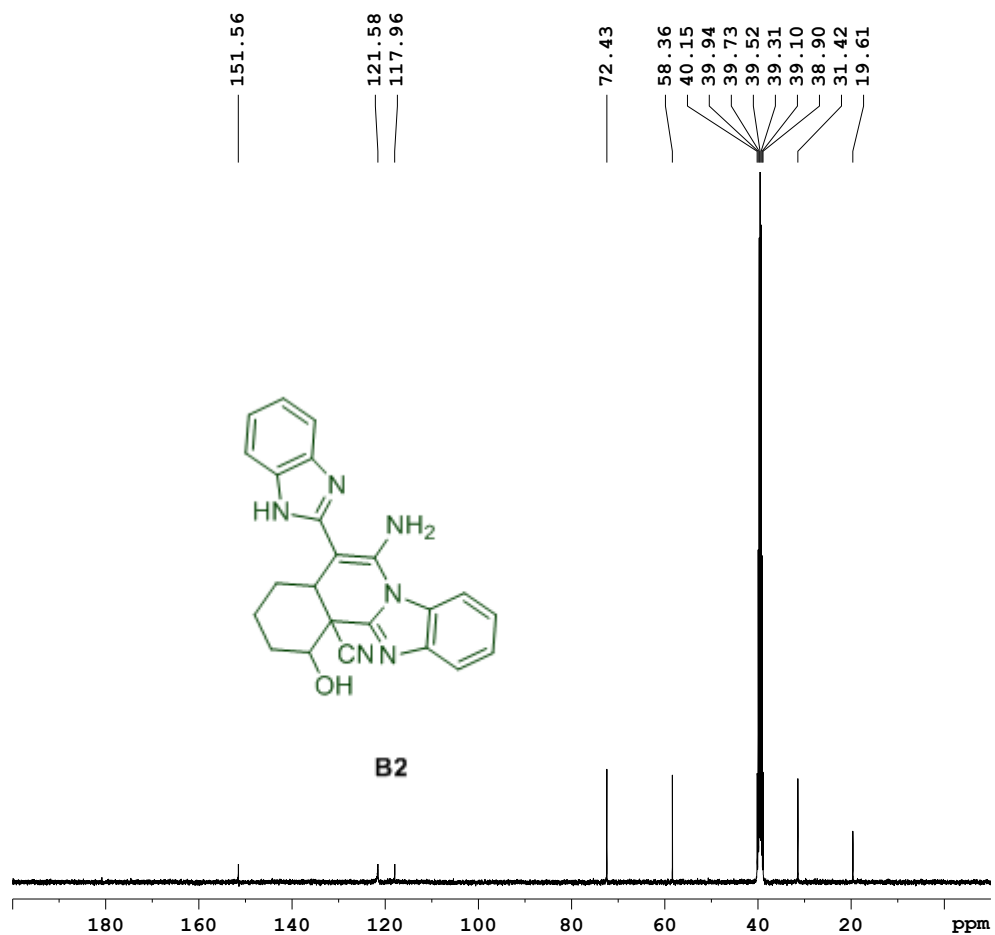
Figure 5 13 C NMR spectra of compound B2.
