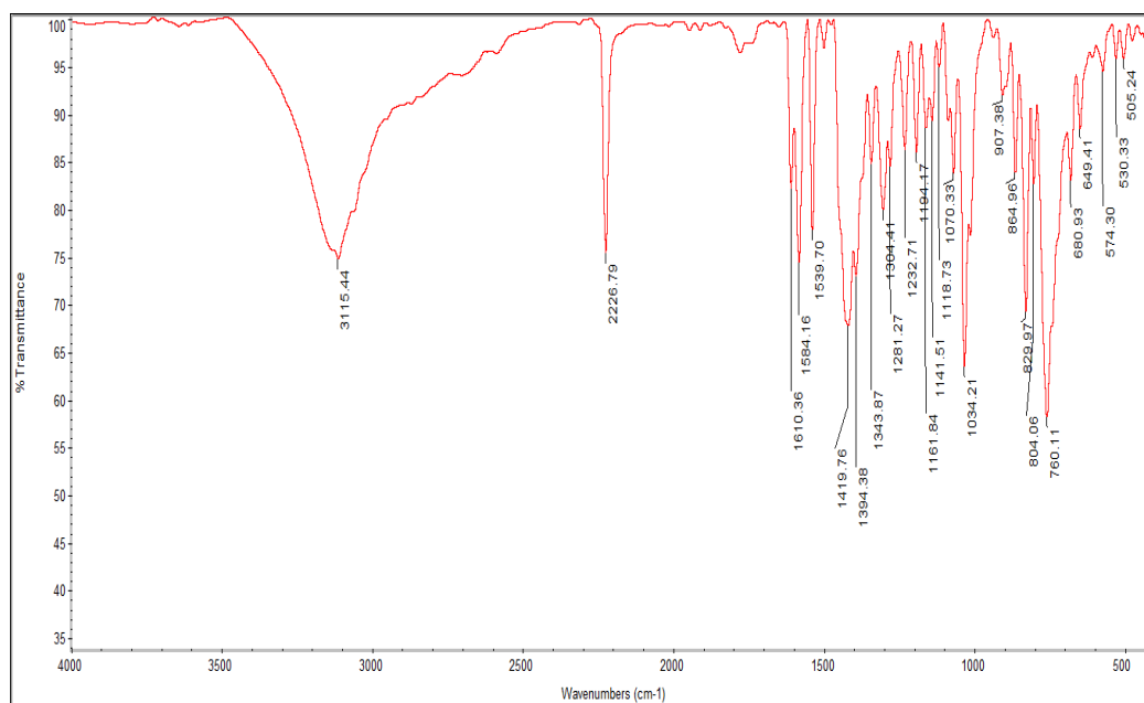
Figure 9 FT-IR spectra of compound B3.
