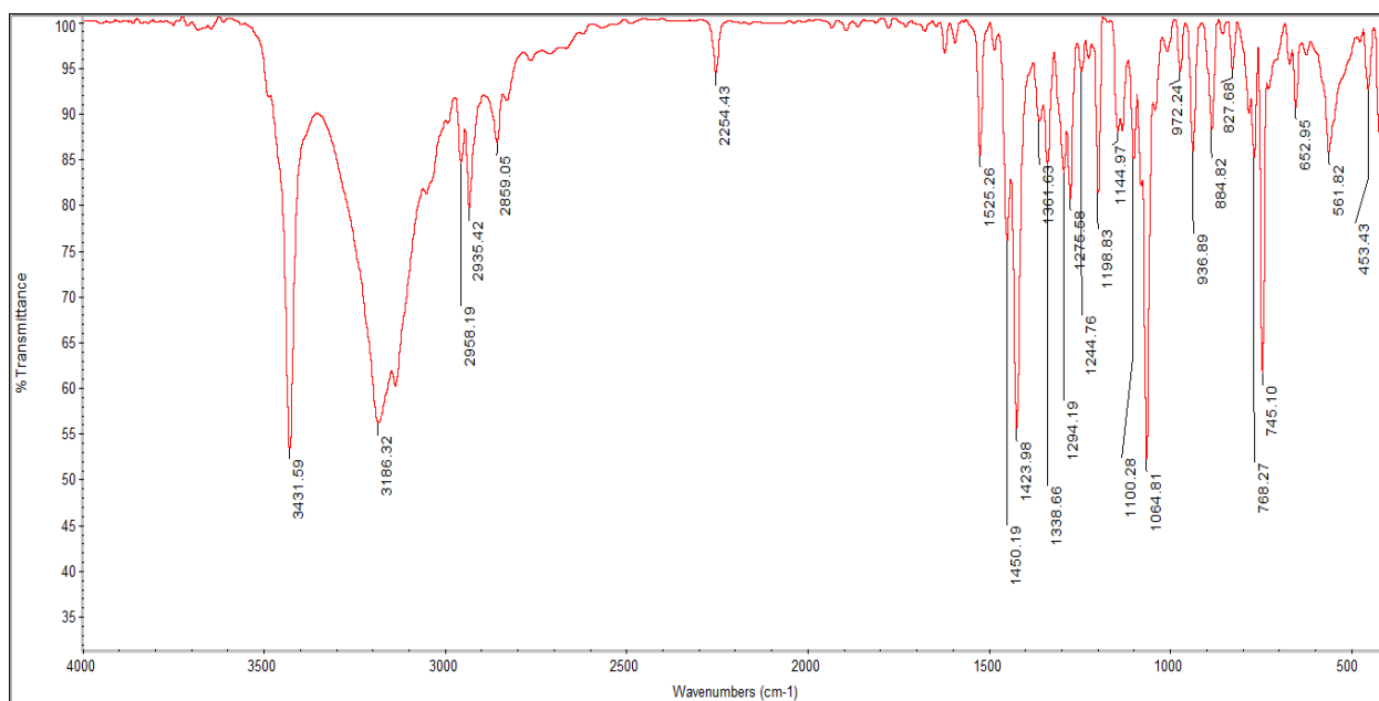
Figure 6 FT-IR spectra of compound B2.
