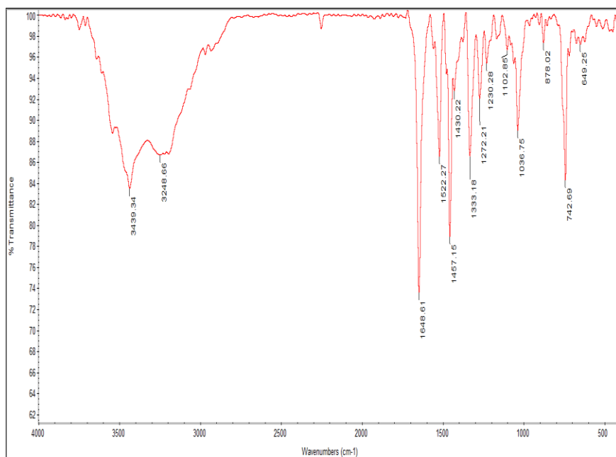
Figure 3 FT-IR spectra of compound B1.
