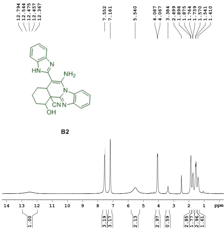
Figure 4 1 H NMR spectra of compound B2.
