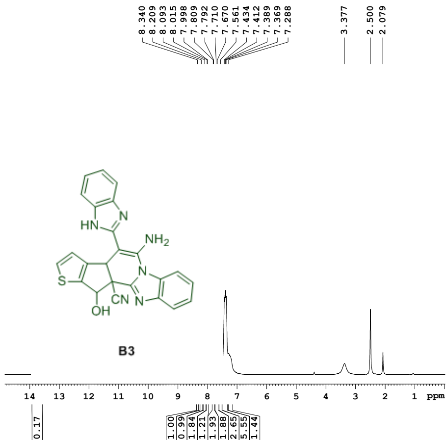
Figure 7 1 H NMR spectra of compound B3.
