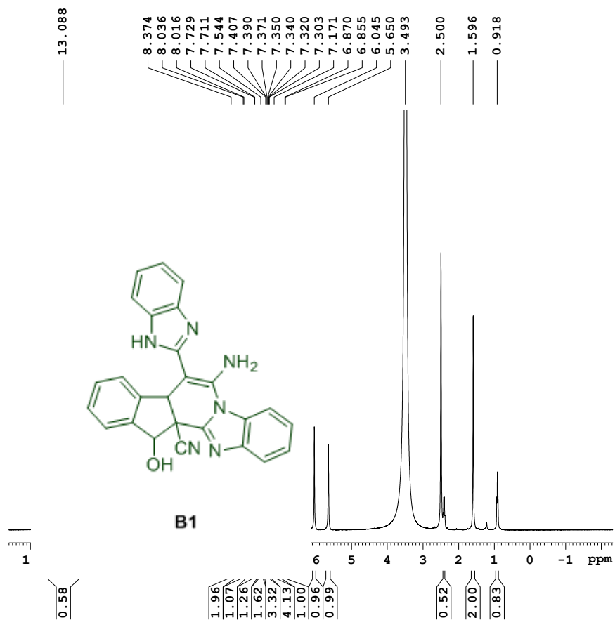
Figure 1 1 H NMR spectra of compound B1.
